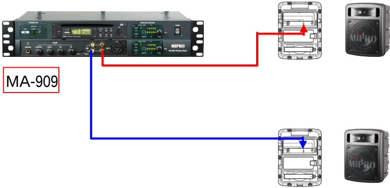
MA-303AXP Line in Application C: MA 303 line out to MA303AXP line in
