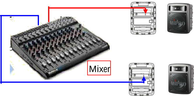
MA-303AXP Line in Application A: Mixer out to MA303AXP line in
